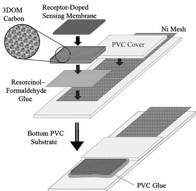
Fig. 1 Schematic setup of a 3DOM carbon-contacted ion-selective electrode
