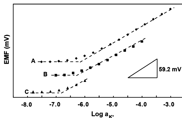
Fig. 2 Potassium ion calibration curves for K^+ -selective ISEs recorded: Conditioning in A 1 mM KCl for 1 day, B 0.1 mM KCl for 1 day, and C 1 \mu M KCl for 1 day. For clarity, response curves have been shifted vertically relative to one another
