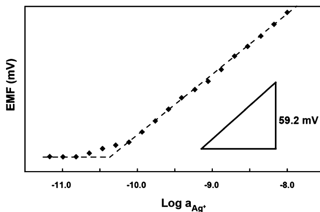
Fig. 3 Silver ion calibration curve for \text{Ag}^+ -selective electrode, with the lowest detection limit achieved in this work, recorded after conditioning in 1 mM \text{AgNO}_3 for 1 day and 1 nM \text{AgNO}_3 for 2 days
